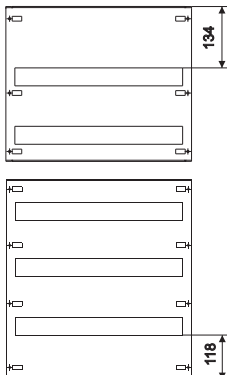
RNB-5N120.. RNB-5N165..
