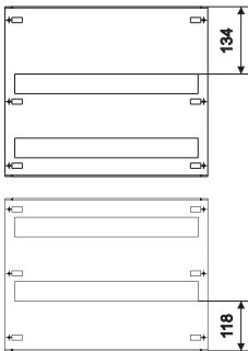
RNB-4N96.. RNB-4N132..
