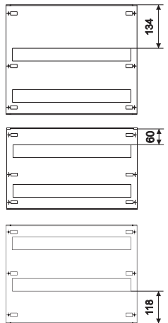
RNB-6N144.. RNB-6N198..
